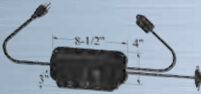
50W LED Power Supply with Photocell
